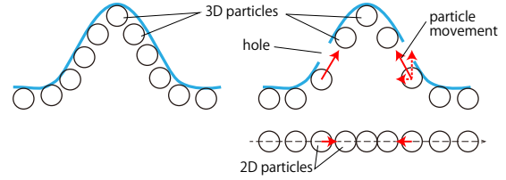
Fig. 4 Holes on surface generated by the vertical movement of the particles. Fully three dimensional simulation generates uniform particle distribution (left), while particle-based SWE causes non-uniform distribution in three dimensional space (right).
