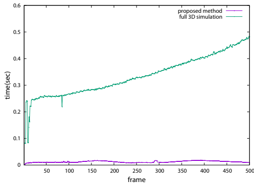
Fig. 9 Comparison of computational time of Scene 1 with full 3D simulation.
