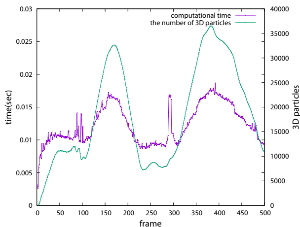
Fig. 10 Computational time of Scene 1 with the number of 3D particles.
