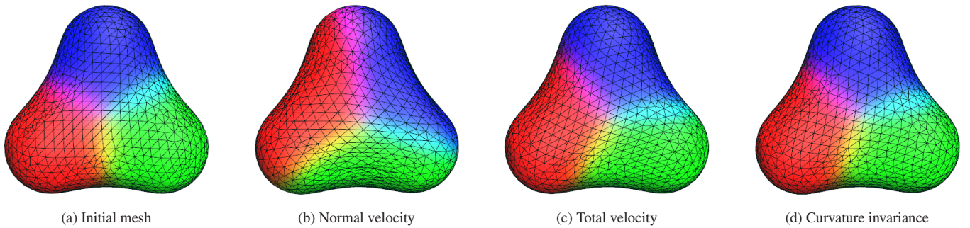
Fig. 7 Rotation of three particles.
