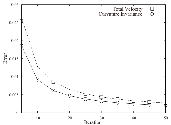
Fig. 9 Average error of vertex position by the number of iterations used for the mesh fairing.
