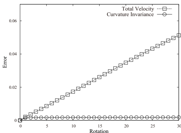
Fig. 10 Average error of vertex position by the number of rotations.
