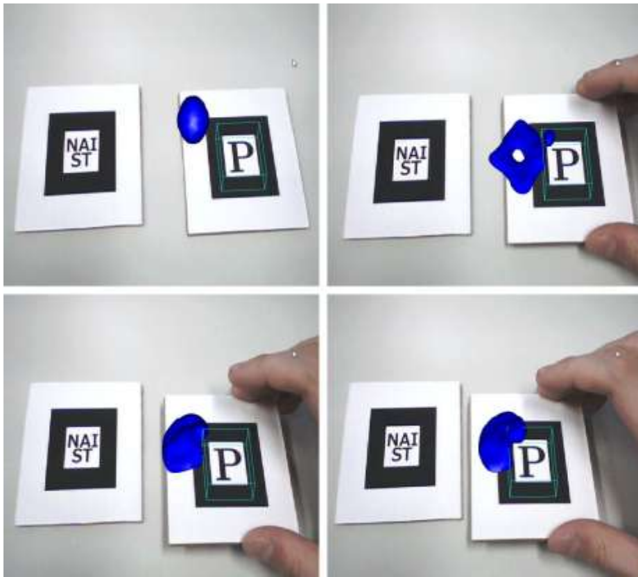
Fig. 2. Water drop interacting with a solid box
